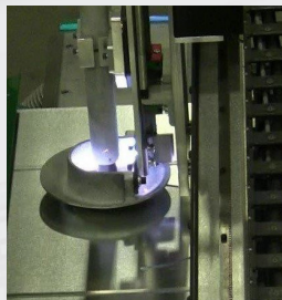
Optional Coil Line Plasma Cutting US Patent #9,393,638 & #9,731,376
