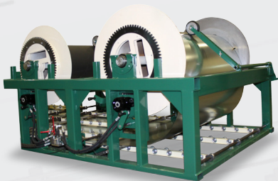
Coil Spool Assembly US Patent #7,673,915
