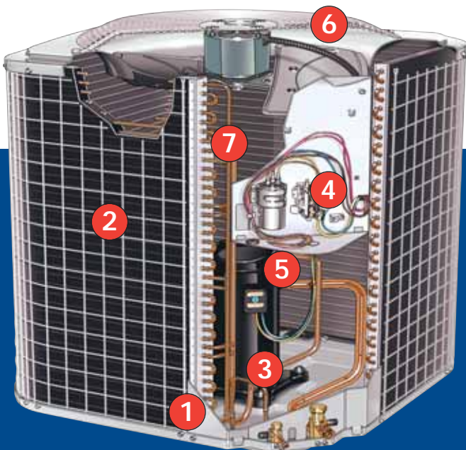
Air Conditioner
